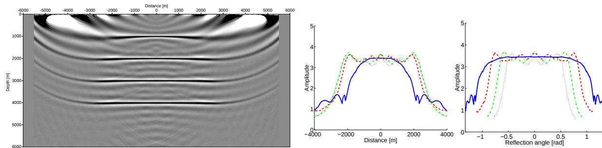
Figure 2: Image using condition (10) (left) and amplitude along reflector images as function of offset (center) and angle (right).
