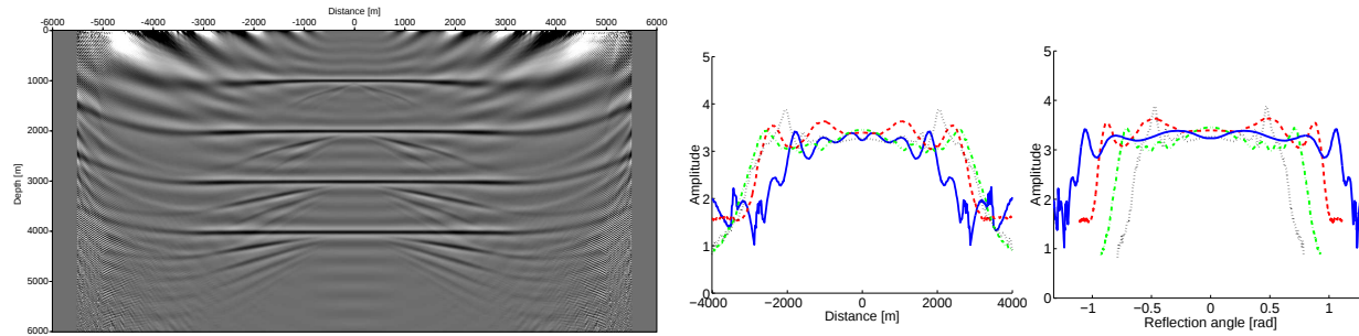
Figure 10: Image using condition (22) (left) and amplitude along reflector images as function of offset (center) and angle (right).
