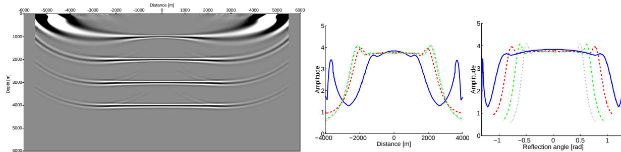
Figure 12: Image using condition (24) (left) and amplitude along reflector images as function of offset (center) and angle (right).
