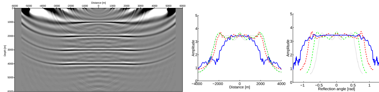
Figure 4: Image using condition (14) with \varepsilon from equation (15) using \lambda = 0.1 (left) and amplitude along reflector images as function of offset (center) and angle (right).
