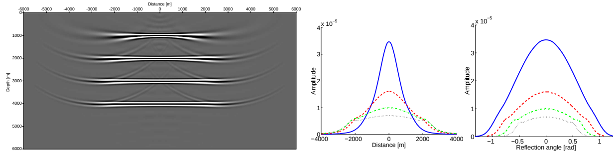
Figure 1: Image using condition (8) (left) and amplitude along reflector images as function of offset (center) and angle (right).
