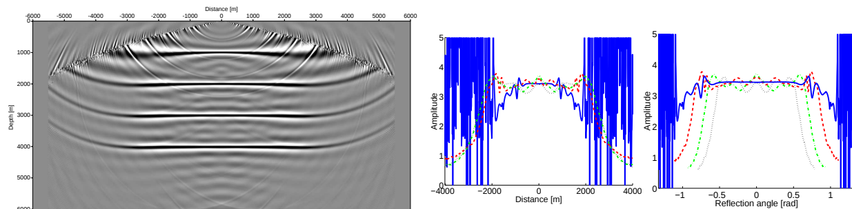
Figure 3: Image using condition (12) (left) and amplitude along reflector images as function of offset (center) and angle (right).
