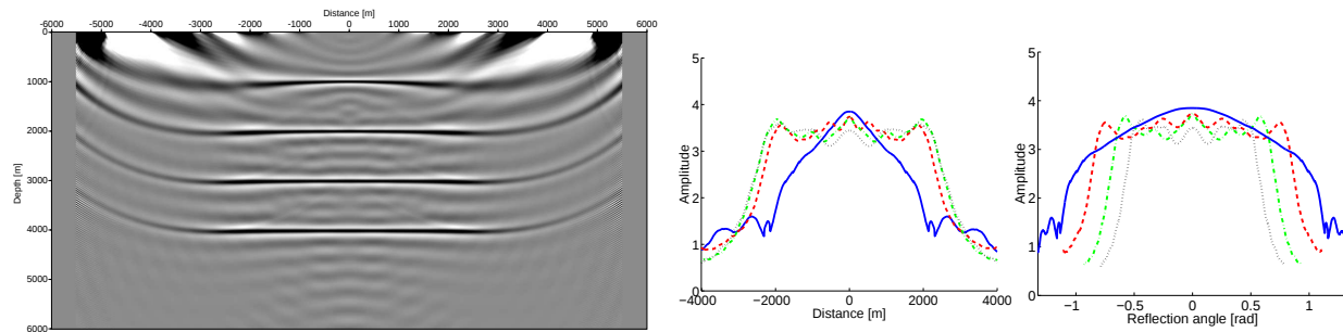
Figure 8: Image using condition (19) (left) and amplitude along reflector images as function of offset (center) and angle (right).
