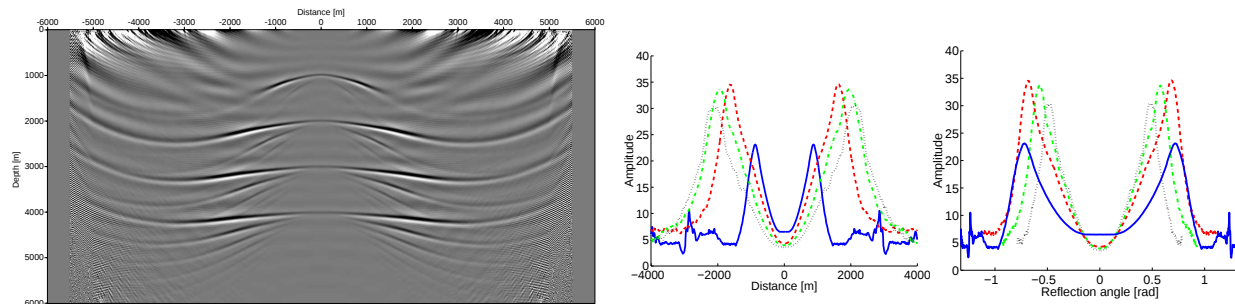
Figure 7: Image using condition (17) with \varepsilon from equation (16) using \lambda = 0.05 (left) and amplitude along reflector images as function of offset (center) and angle (right).
