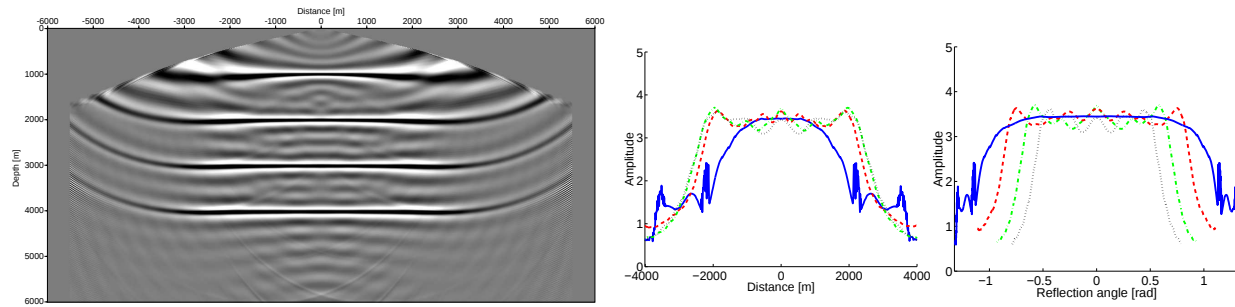
Figure 6: Image using condition (17) with \varepsilon from equation (15) using \lambda = 0.1 (left) and amplitude along reflector images as function of offset (center) and angle (right).
